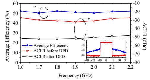
Fig. 6. The measured average efficiency and ACLR before and after DPD using modulated signal and measured spectrum at 1.9 GHz.
